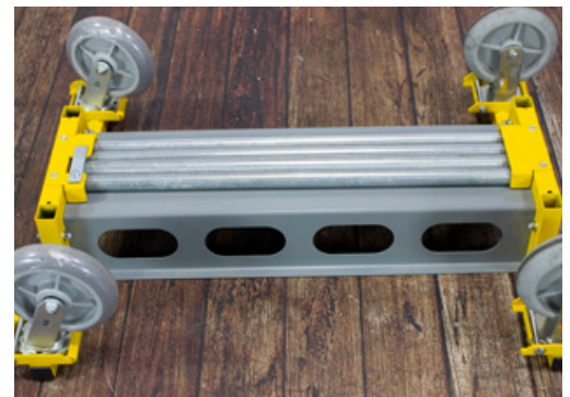
Posts store on the underside of the cart.
